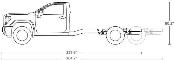
SIERRA CHASSIS CAB REGULAR CAB
